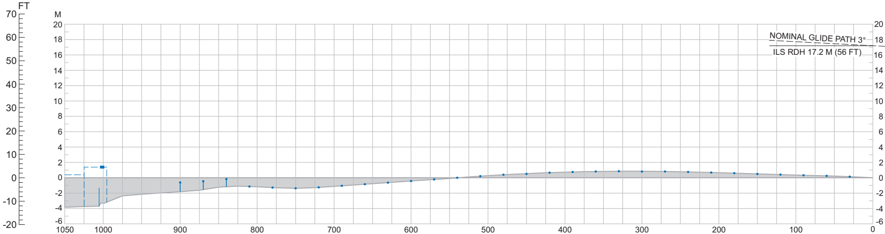
Contours and HGT are related to ELEV of THR RWY 12R
